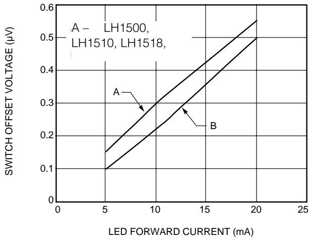
A. Switch Offset Voltage vs. LED Current
