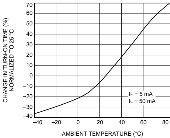
E. Turn-On Time vs. Temperature (LH1541)
