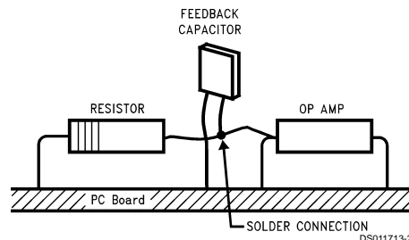
FIGURE 11. Air Wiring
