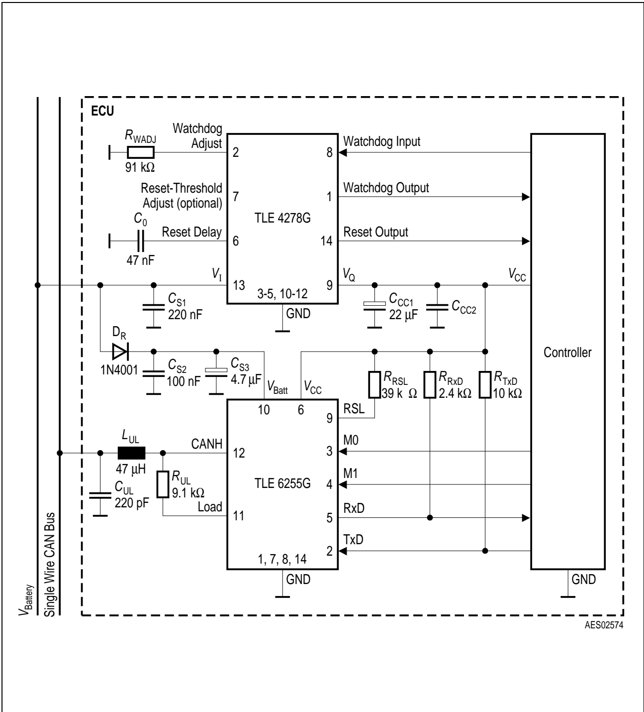
Figure 9 Application Circuit
