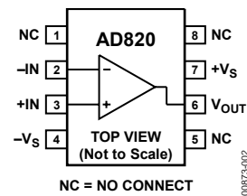
Figure 2. 8-Lead SOIC
