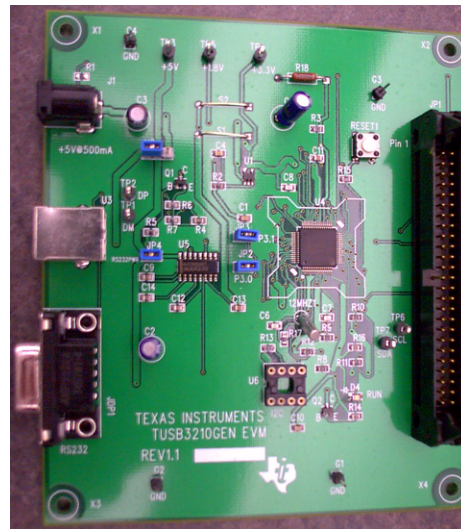
Figure 8. Generic EVM
