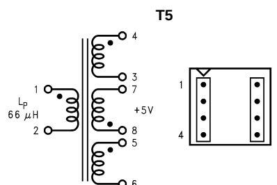
Figure 19. Coilcraft Q4338-B (Top View)
