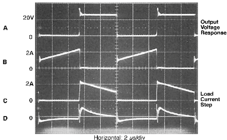
Figure 8. Switching Waveforms
