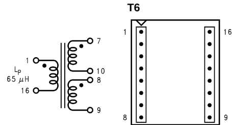
Figure 23. Pulse PE-68414 (Surface Mount) (Top View)
