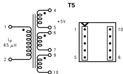
Figure 30. Schott 67140890 (Top View)
