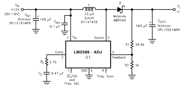
Figure 35. +12V to +24V Boost Regulator
