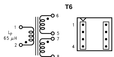
Figure 17. Coilcraft Q4339-B (Top View)
