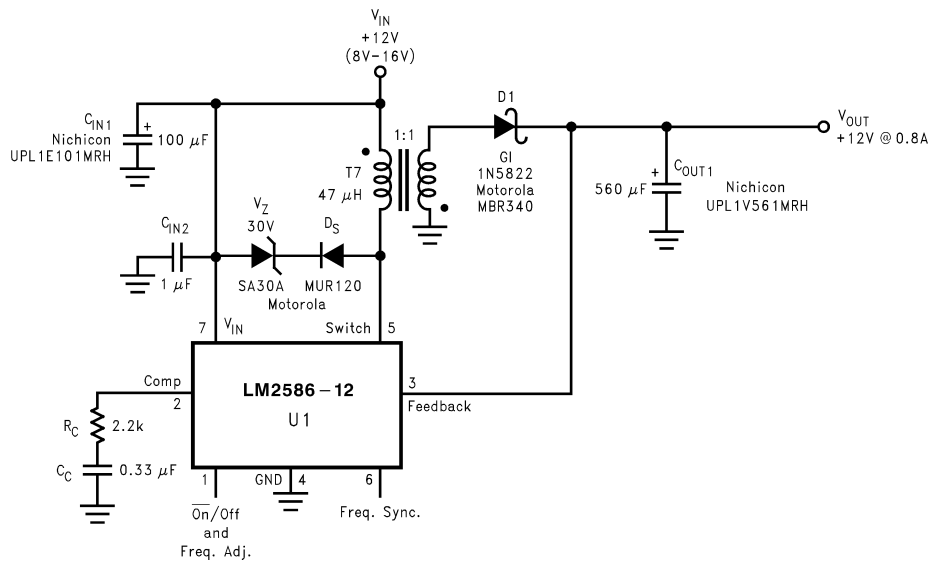
Figure 12. Single-Output Flyback Regulator
