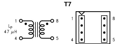
Figure 23. Pulse PE-68414 (Surface Mount) (Top View)
