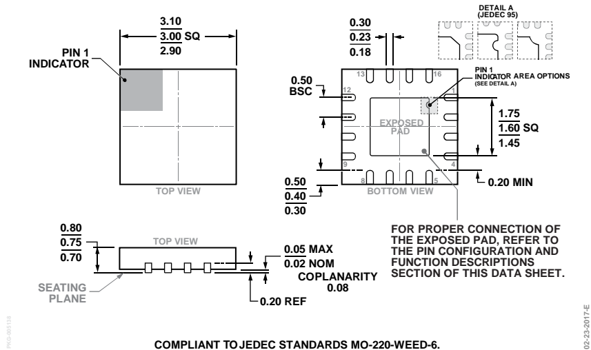
Figure 43. 16-Lead Lead Frame Chip Scale Package [LFCSPP] 3 mm x 3 mm Body and 0.75 mm Package Height (CP-16-22)
