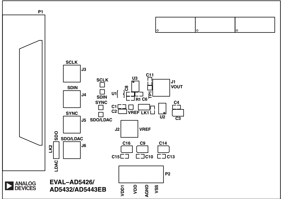
Figure 20. Silkscreen—Component Side View (Top Layer)
