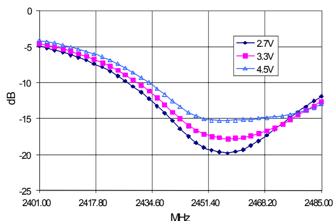
Figure 10: Output Match (SE) vs. Frequency and Voltage
