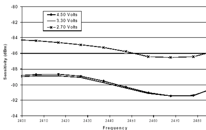
Figure 8: RX Sensitivity (12.5% BER) vs. Frequency
