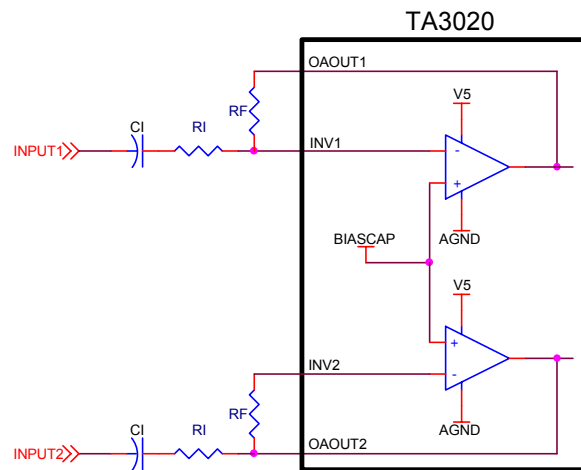
Figure 2: Input Stage
