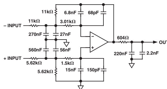
Figure 23. Recommended External Analog Filter for Sub Channel
