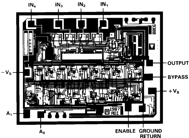
METALIZATION PHOTOGRAPH
