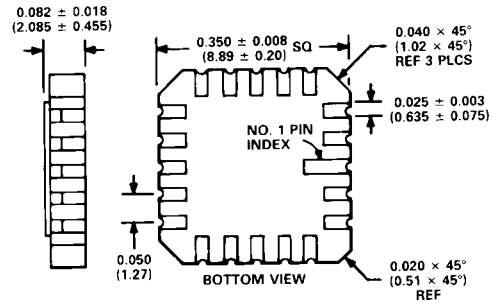
20-Pin LCC (E) Package
