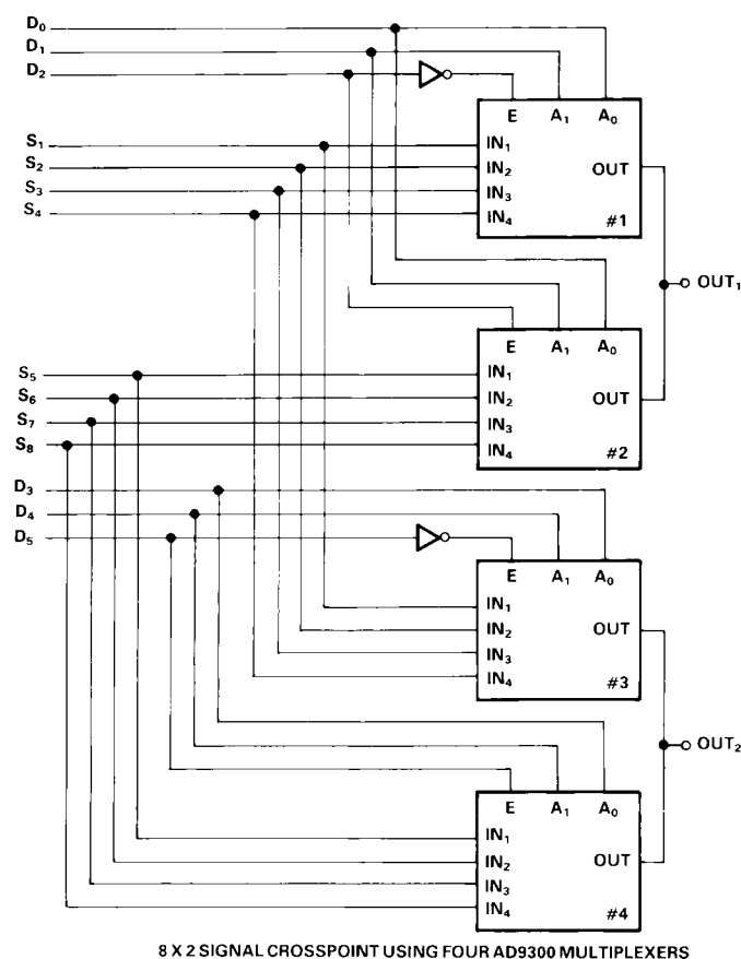
Figure 11. 8 \times 2 Signal Crosspoint Using Four AD9300 Multiplexers
