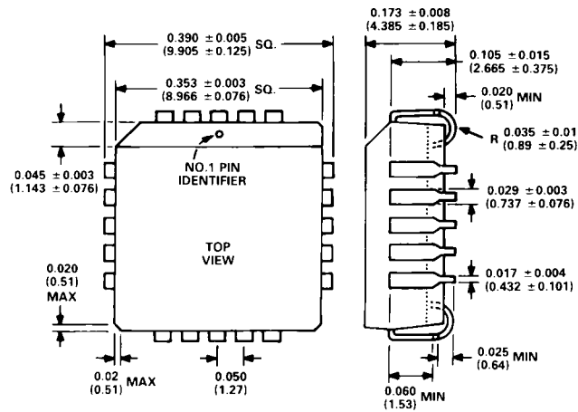
20-Pin PLCC (P) Package
