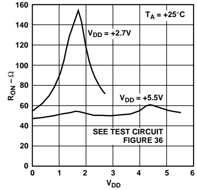
Figure 25. AD8403 Incremental Wiper ON Resistance vs. V DD
