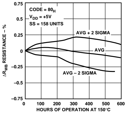
Figure 14. Long-Term Drift Accelerated by Burn-In
