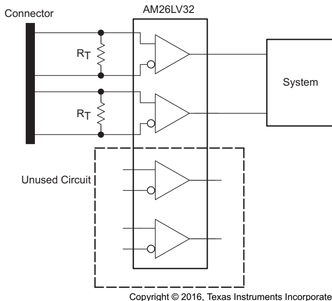
Figure 14. Typical Application With Unused Receivers
