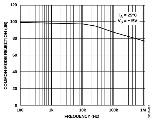
Figure 25. OP292/OP492 CMR vs. Frequency @ \pm 15\text{V}
