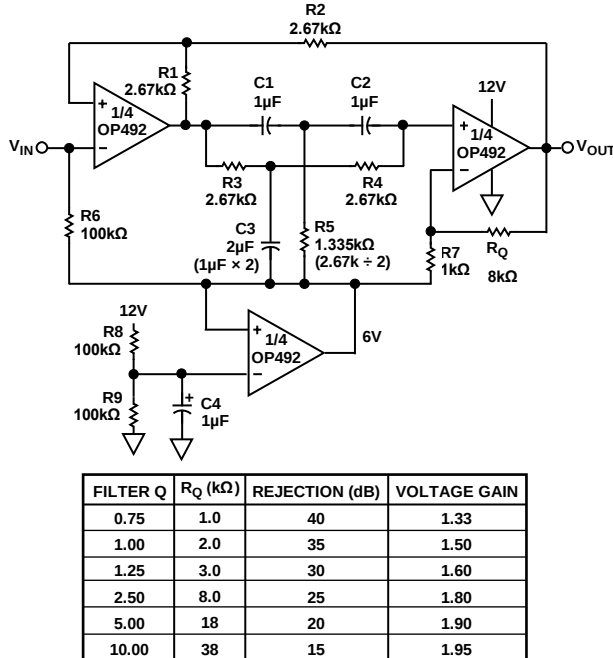
Figure 39. Single-Supply 50 Hz/60 Hz Notch Filter
