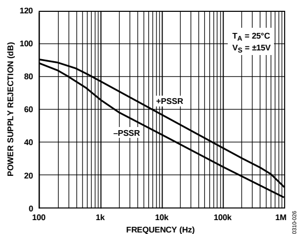
Figure 26. OP292/OP492 PSR vs. Frequency @ \pm 15\text{V}
