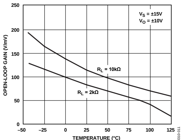
Figure 11. OP292 Open-Loop Gain vs. Temperature @ \pm 15 V
