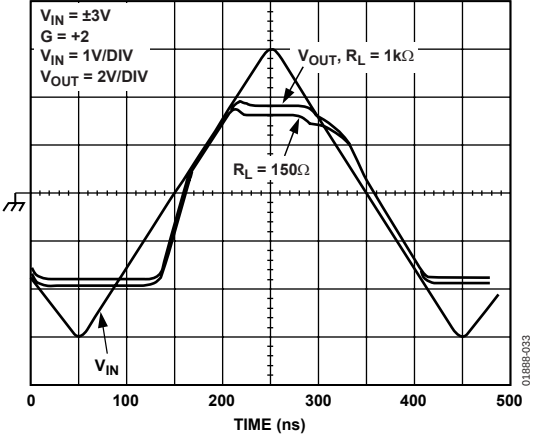
Figure 33. Overdrive Recovery vs. R_L (See Figure 49)
