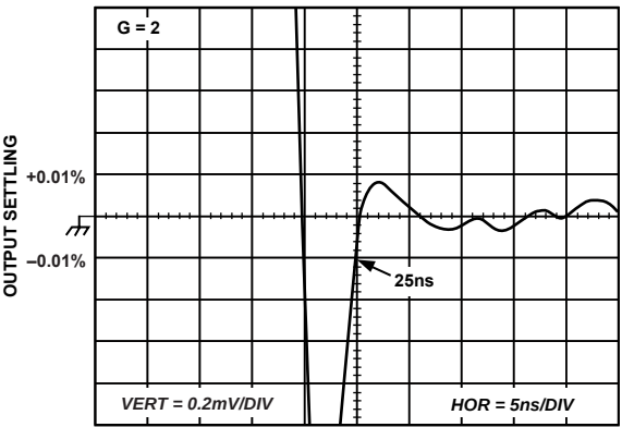
Figure 34. 0.01% Settling Time, 2 V Step
