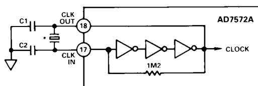
Figure 6. AD7572A Internal Clock Circuit
