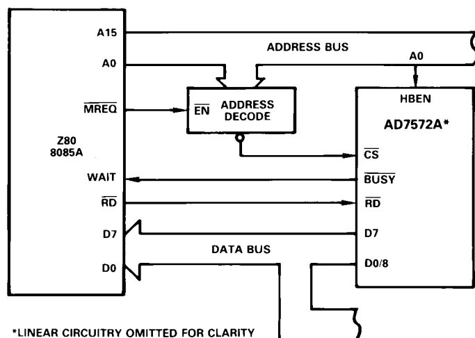
Figure 22. AD7572A-8085/Z80 Interface
