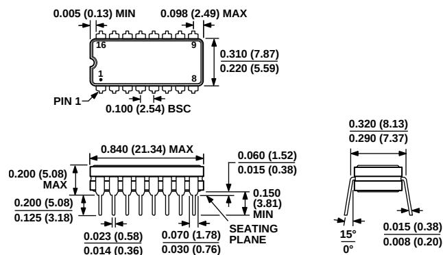
Figure 58. 16-Lead Ceramic Dual In-Line Package [CERDIP] (Q-16)
