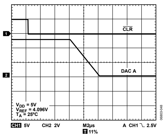
Figure 37. Hardware \overline{\text{CLR}}
