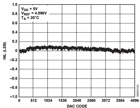
Figure 9. AD5044 INL
