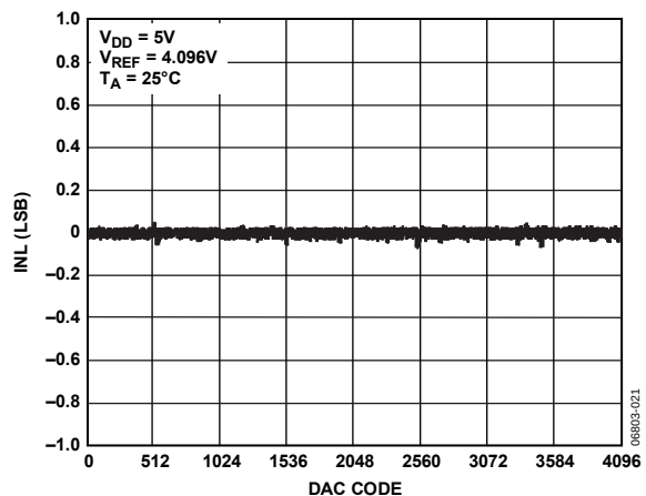
Figure 10. AD5024 INL
